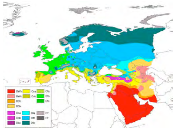
Köppen-Geiger European classification
