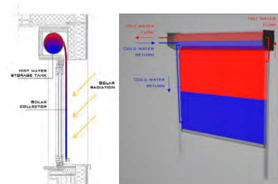
► Fig. 3: Thermosyphon water circulation
