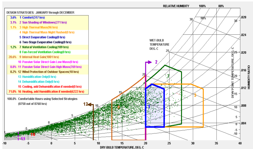
Psychrometric conditions
