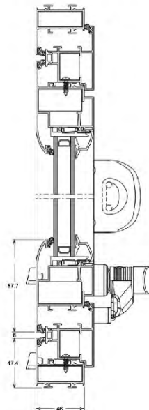
Section detail of windows frame
