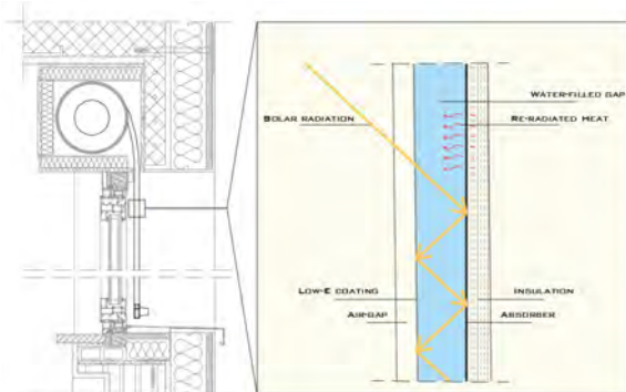
► Fig. 1: System's components and thermodynamic processes
